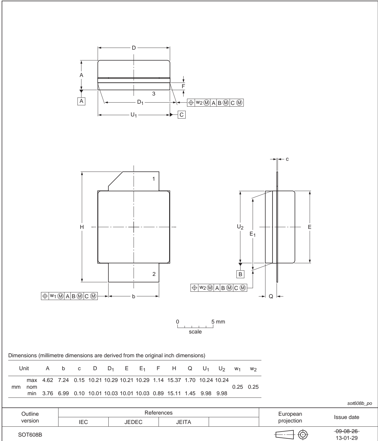
Fig 12. Package outline SOT608B
